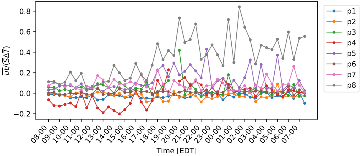
Figure C.4: Normalized covariance between the x wind velocity component and ultrasonic temperature over a diurnal cycle.
