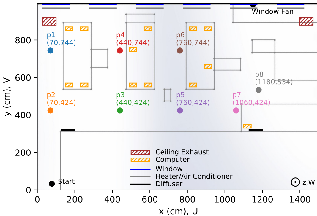
Figure 5.1: Map of the Mechatronics lab with robot start location, positions to measure the environment, and the position of the window fan.
