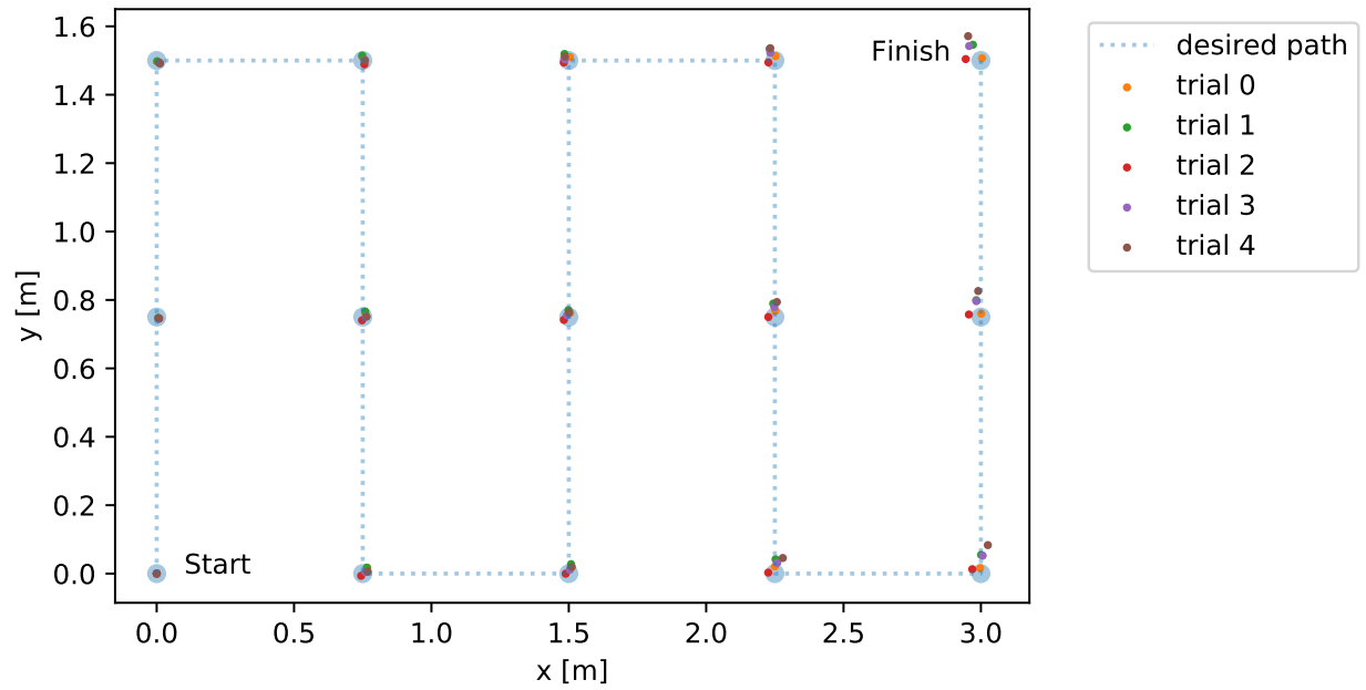
Figure 4.8: Position of the robot at each test point over the path moving in the positive x direction after drift compensation.
