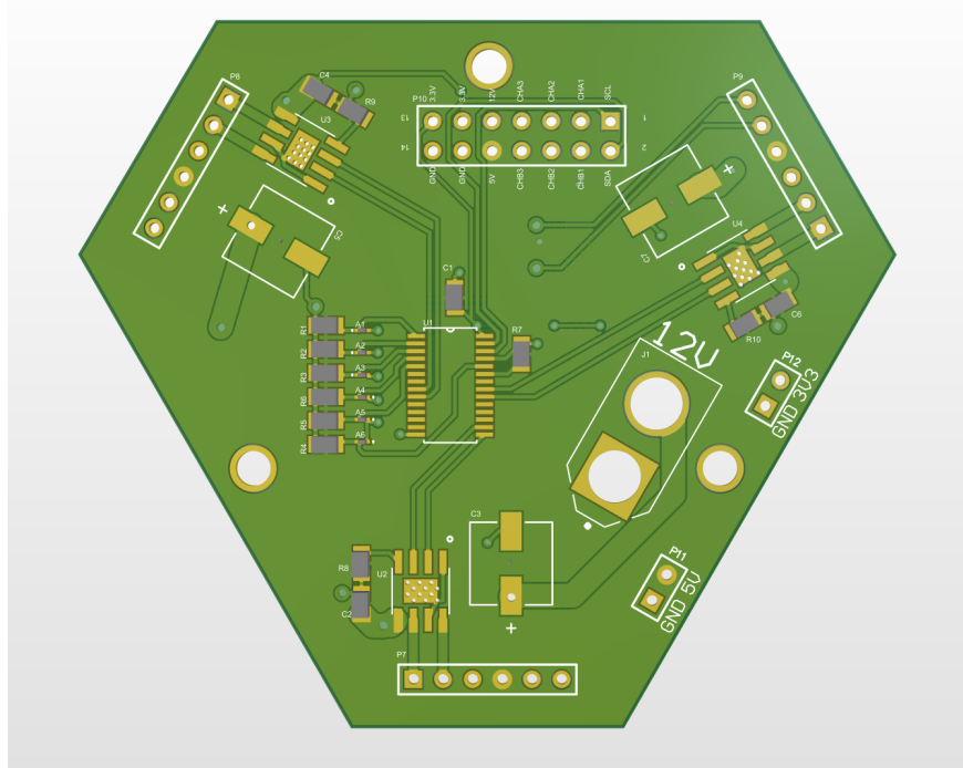
Figure 3.5: Motor driver PCB layout.
