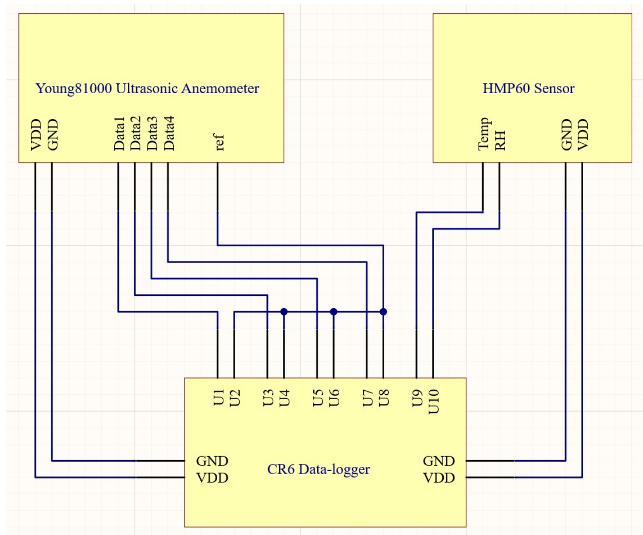
Figure C.6: Wiring diagram of Young81000 ultrasonic anemometer, HMP60 temperature and relative humidity sensor, and CR6 data-logger.
