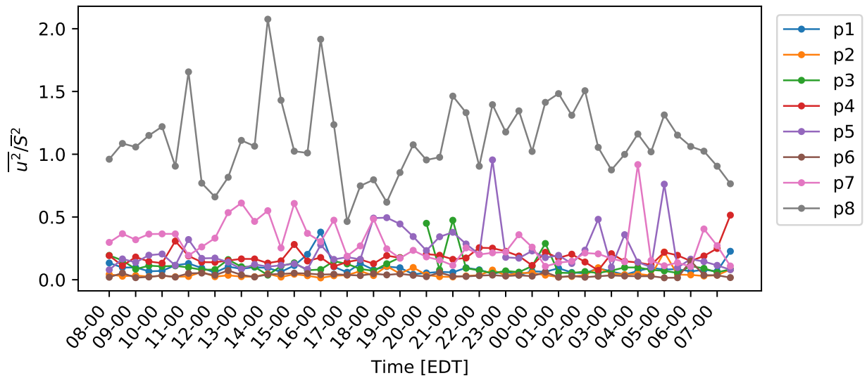
Figure 5.9: Normalized wind velocity vector variance in the x direction over a diurnal cycle.
