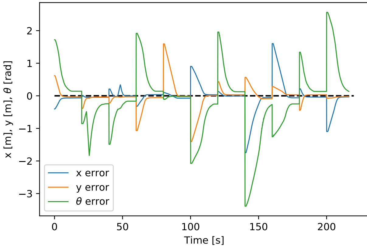
Figure 4.12: Feedback linearization controller error in translational and rotational positions as a function of time when stabilizing to random positions.
