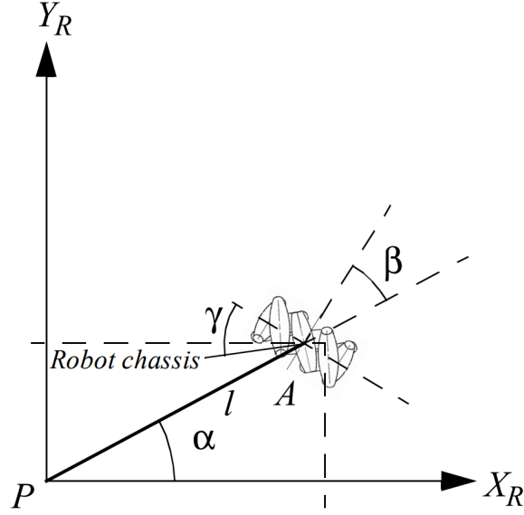
Figure 4.1: Diagram of a Swedish wheel and its corresponding coordinates in the robot's frame of reference (Siegwart et al., 2011).
