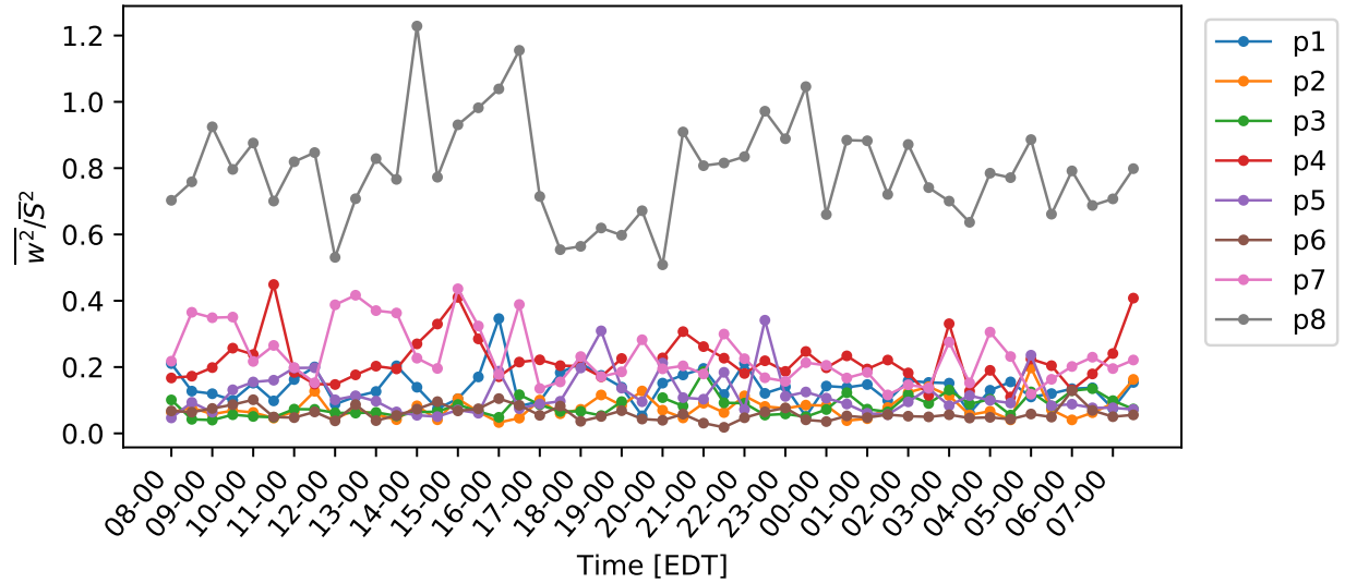
Figure 5.11: Normalized wind velocity vector variance in the z direction over a diurnal cycle.
