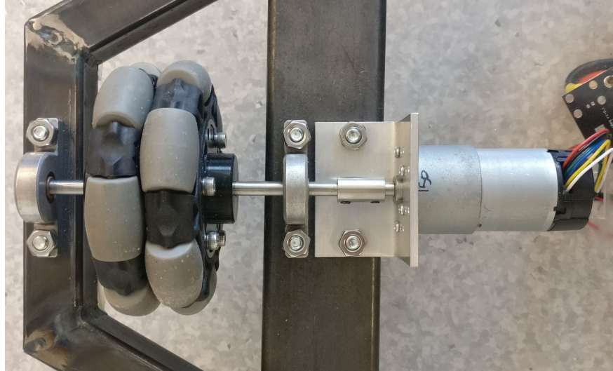
Figure 3.3: View of the wheel drive from the bottom of ARES.
