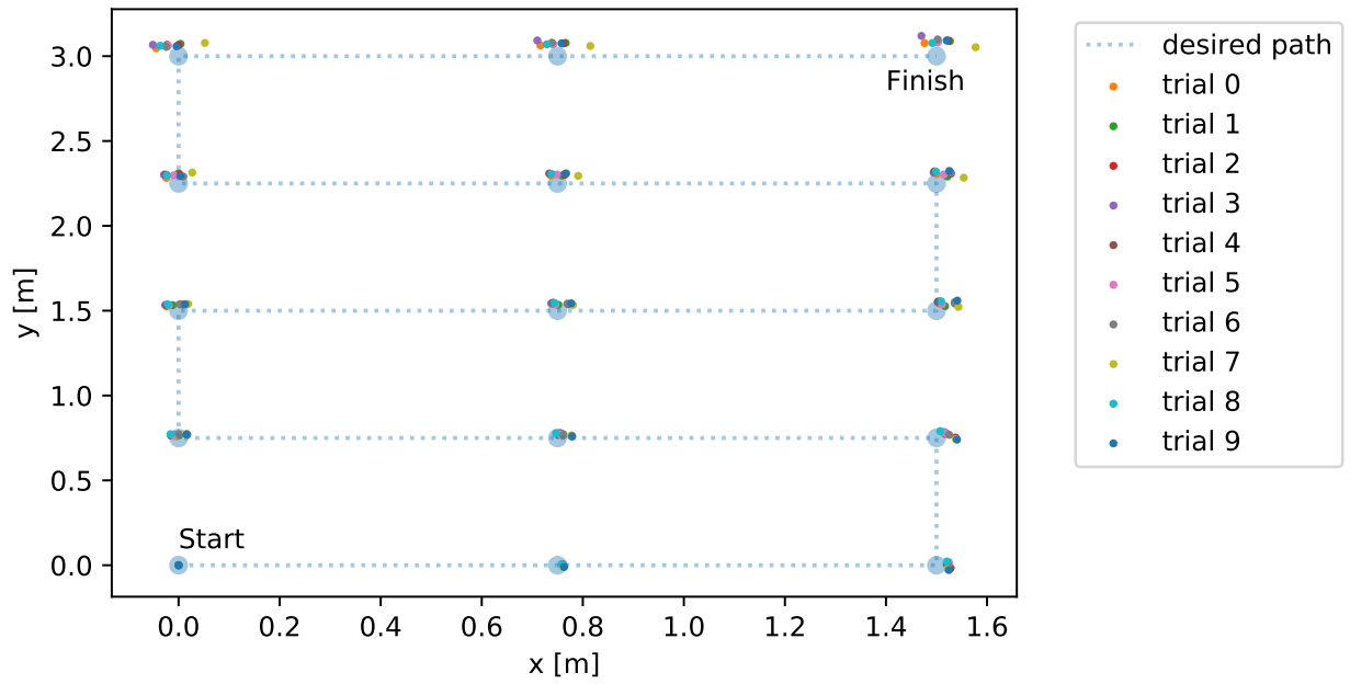
Figure 4.6: Position of the robot at each test point over the path moving in the positive y direction.
