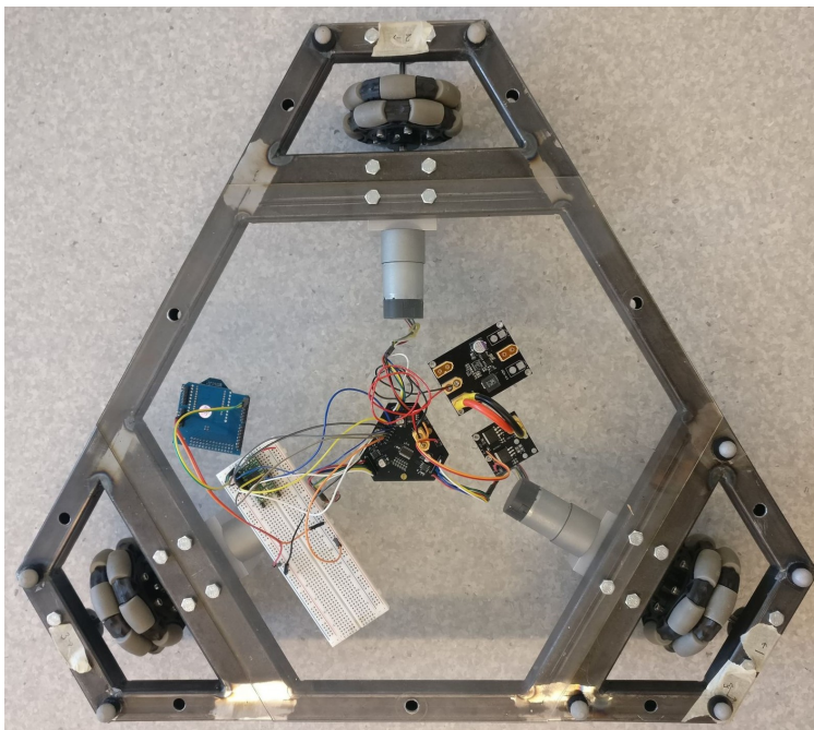
Figure 3.2: Top-down view of ARES' frame with electronics and wheel drives attached.
