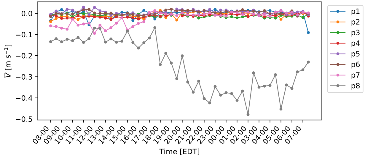
Figure 5.3: Average V component of the wind velocity vector over a diurnal cycle.
