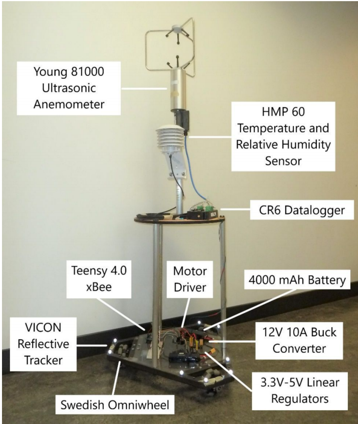
Figure 3.1: ARES set up for thermal comfort measurements.
