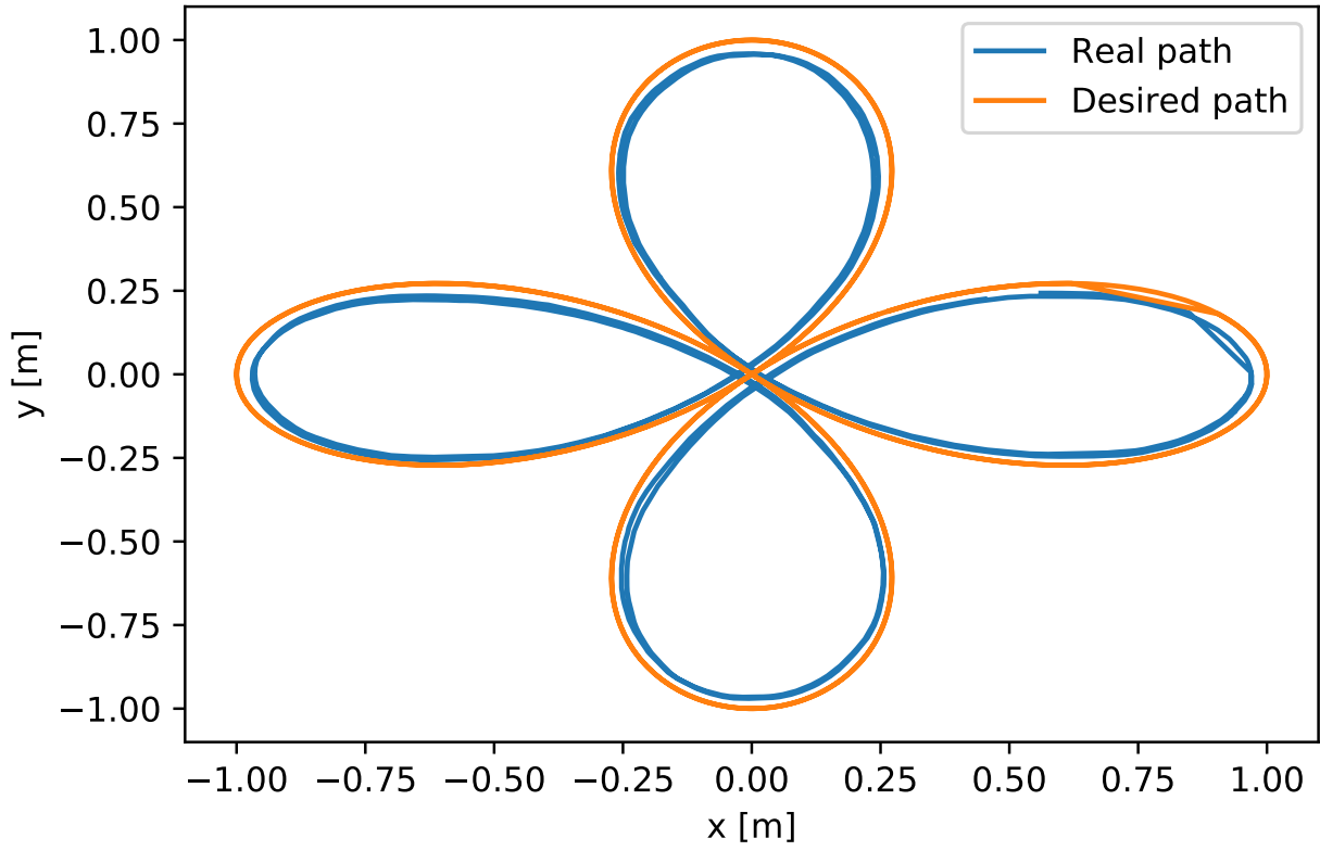
Figure 4.10: Omniwheel robot path compared to desired path using Feedback Linearization.
