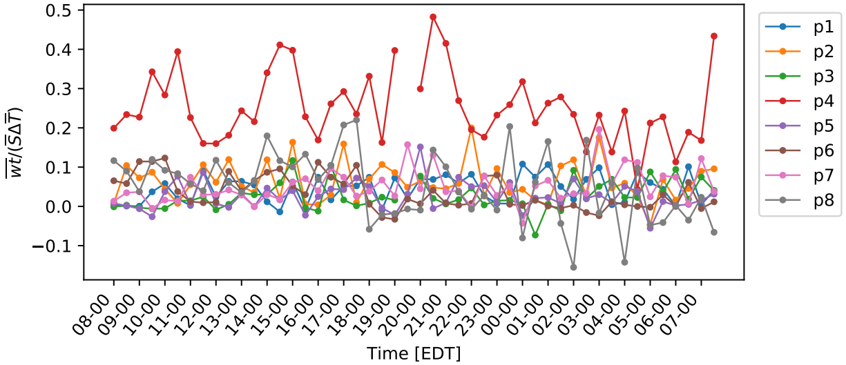
Figure 5.14: Normalized covariance between the wind velocity in the z direction and ultrasonic temperature over a diurnal cycle.
