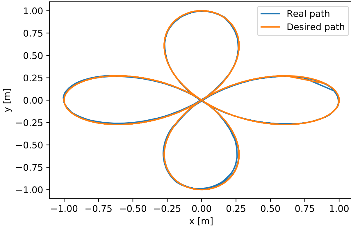
Figure 4.11: Omniwheel robot path compared to desired path using SMC.
