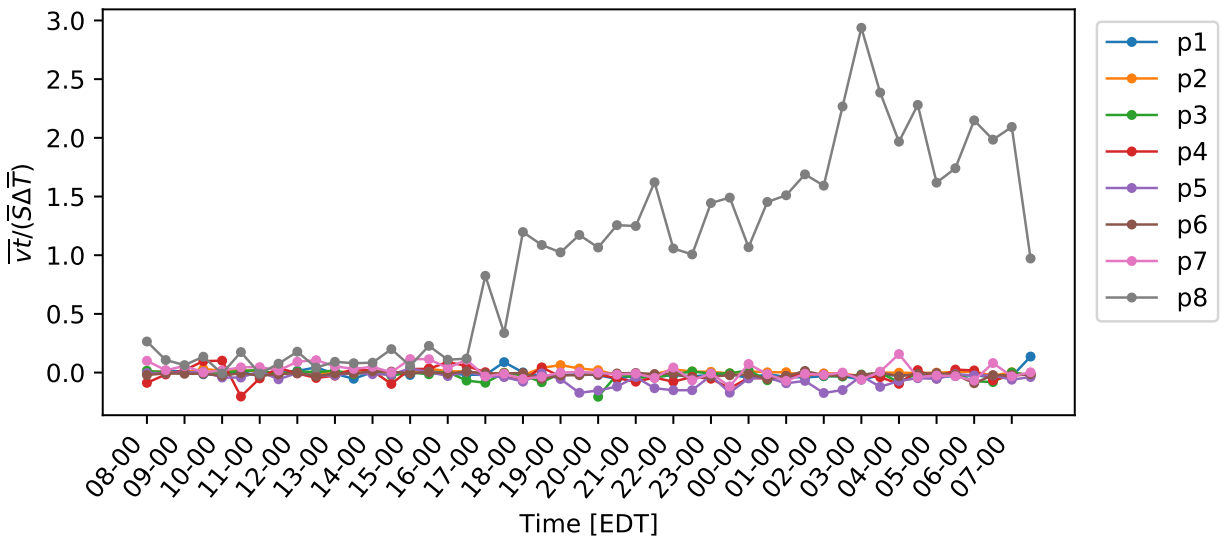
Figure C.5: Normalized covariance between the y wind velocity component and ultrasonic temperature over a diurnal cycle.
