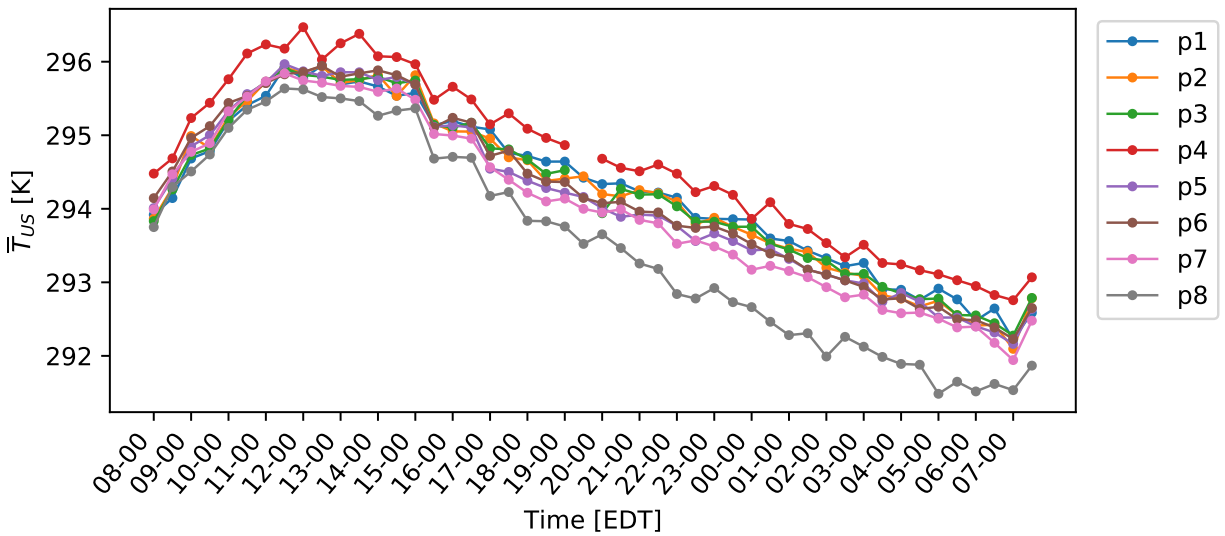
Figure 5.5: Average ultrasonic temperature over a diurnal cycle.
