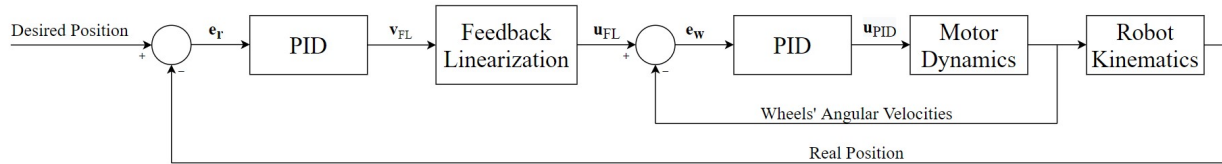
Figure 4.2: Block diagram of feedback linearization controller with a PID controller on each wheel.
