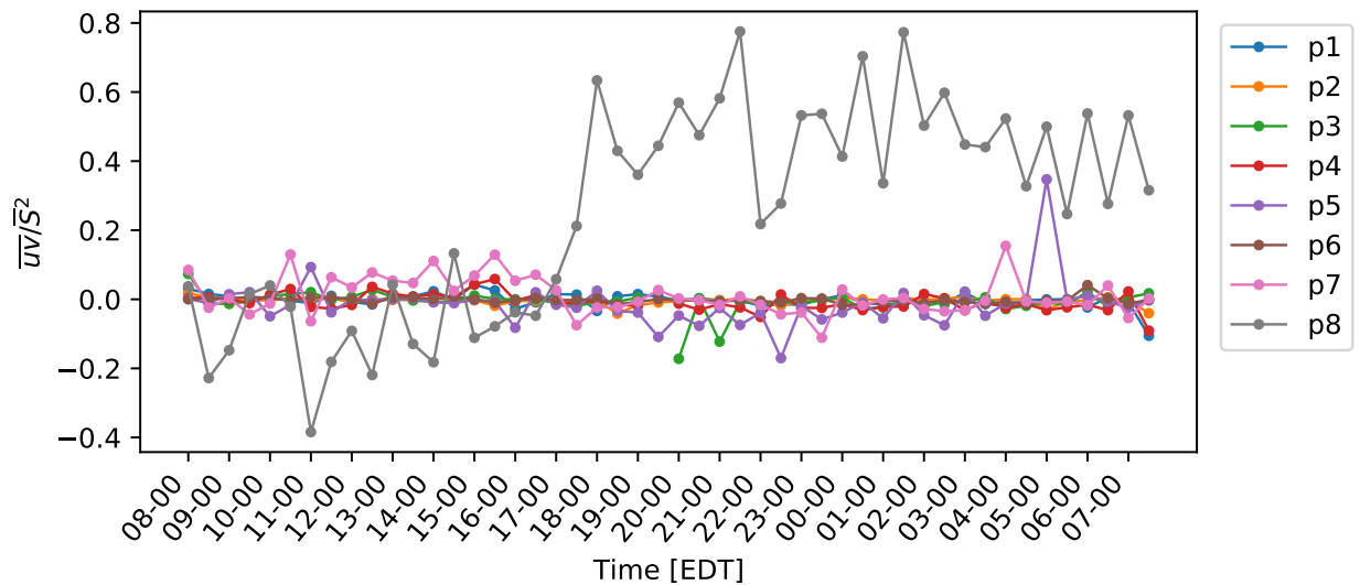
Figure C.1: Normalized covariance between x and y wind velocity components over a diurnal cycle.
