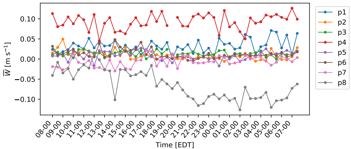
Figure 5.4: Average W component of the wind velocity vector over a diurnal cycle.
