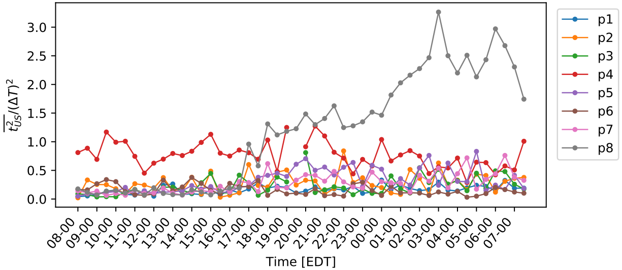
Figure 5.12: Normalized ultrasonic temperature variance over a diurnal cycle.
