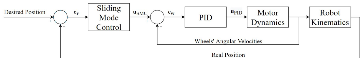
Figure 4.3: Block diagram of sliding mode controller with a PID controller on each wheel.
