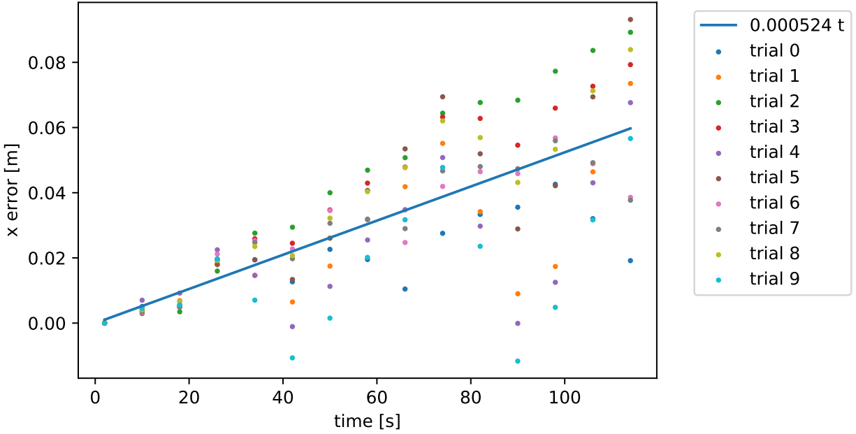
Figure 4.5: Error as a function of time, linear fit shows positional error as a function time corresponding to a drift of 0.0199 \text{ m m}^{-1} .
