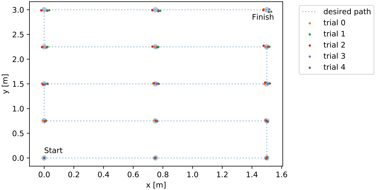
Figure 4.9: Position of the robot at each test point over the path moving in the positive y direction after drift compensation.
