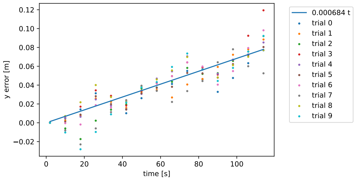
Figure 4.7: Error as a function of time, linear fit shows positional error as a function time corresponding to a drift of 0.0259 \text{ m m}^{-1} .
