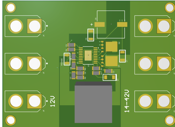
Figure 3.4: 12V DC Buck Converter PCB layout.
