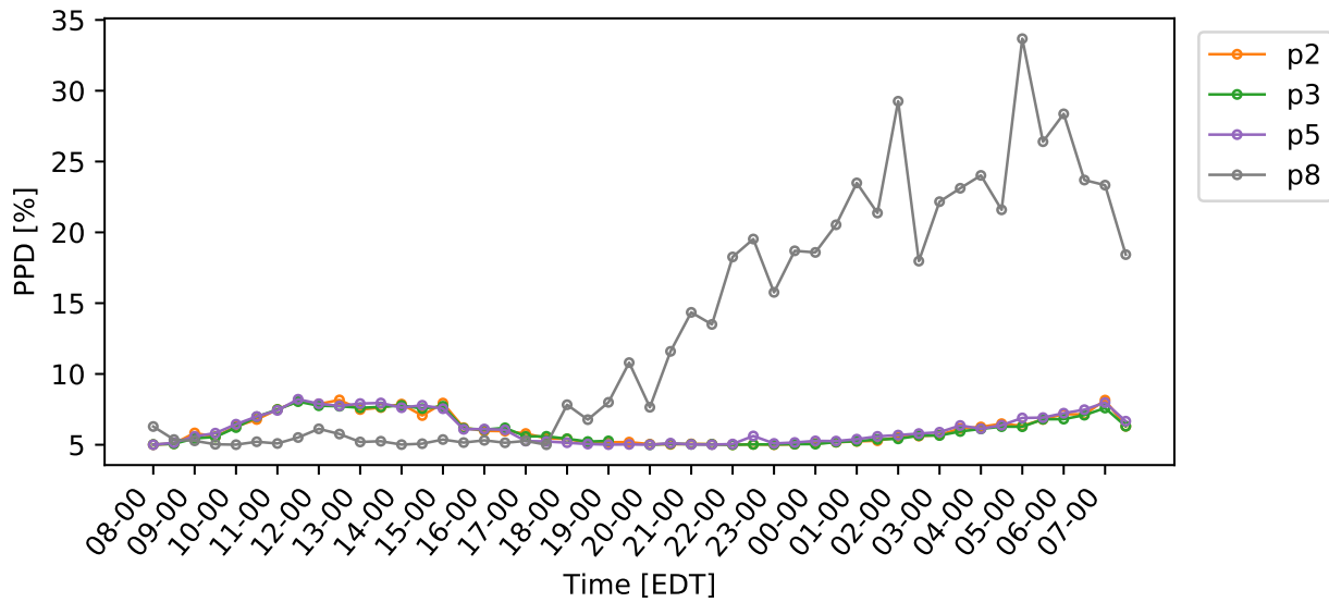
Figure 5.22: PDD with metabolism = 1.7 met and clothing = 0.57 clo over a diurnal cycle.
