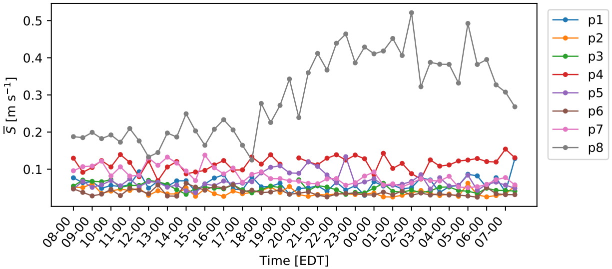
Figure 5.6: Average wind speed over a diurnal cycle.
