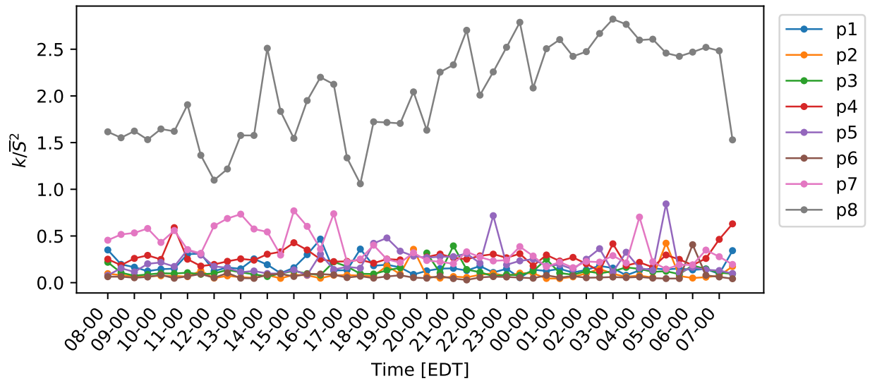
Figure 5.13: Normalized turbulent kinetic energy over a diurnal cycle.
