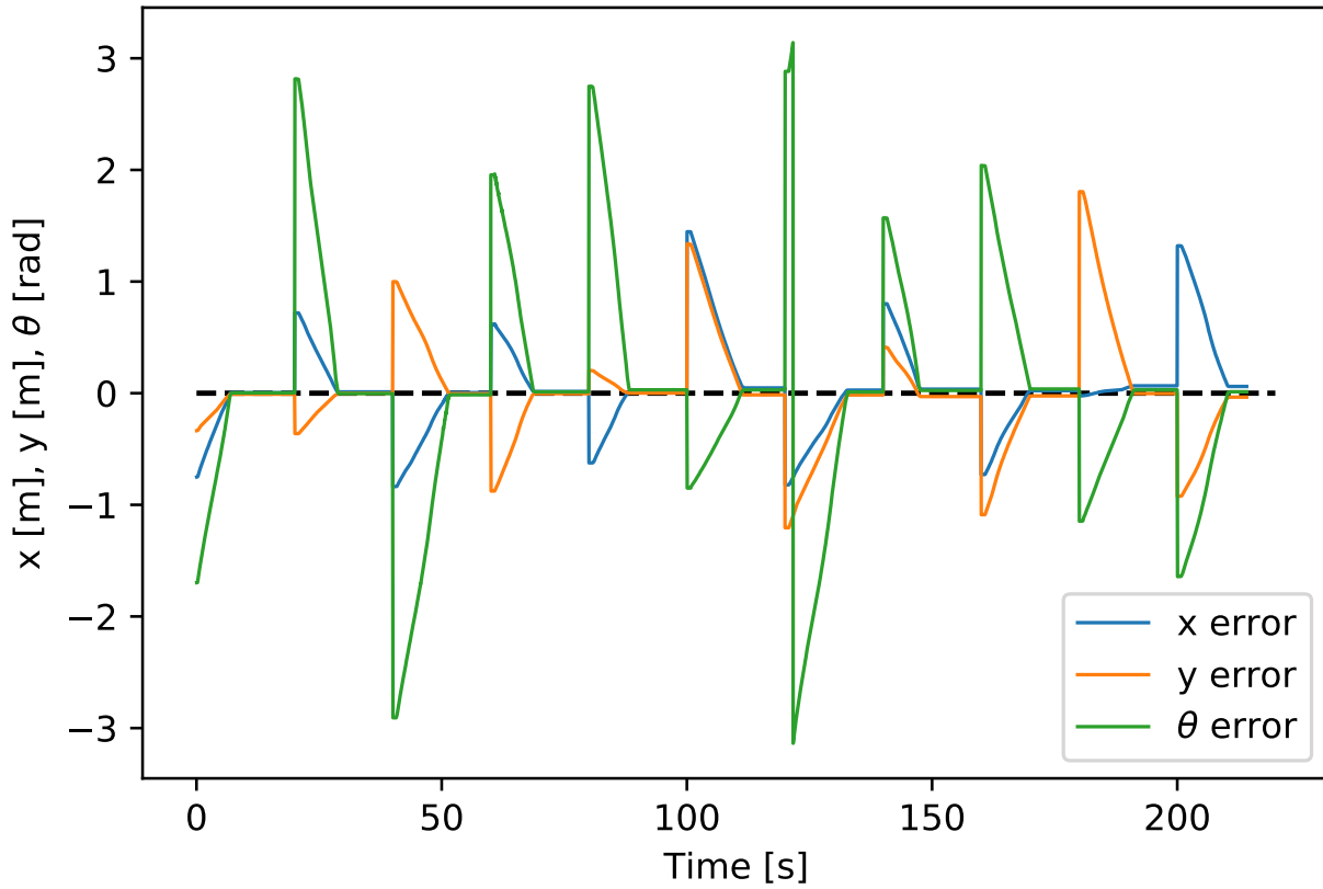
Figure 4.13: Sliding mode controller error in position as a function of time when stabilizing to random positions.
