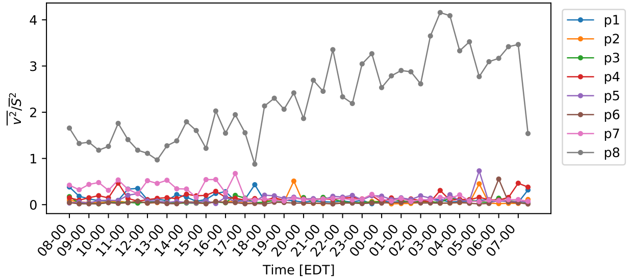
Figure 5.10: Normalized wind velocity variance in the y direction over a diurnal cycle.
