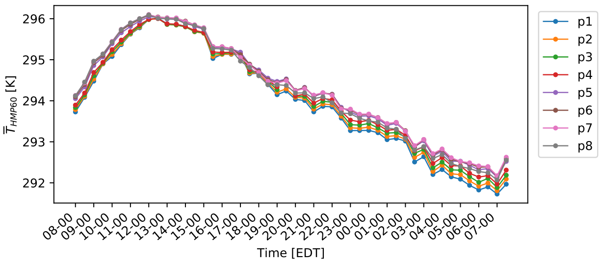
Figure 5.7: Average HMP60 temperature over a diurnal cycle.
