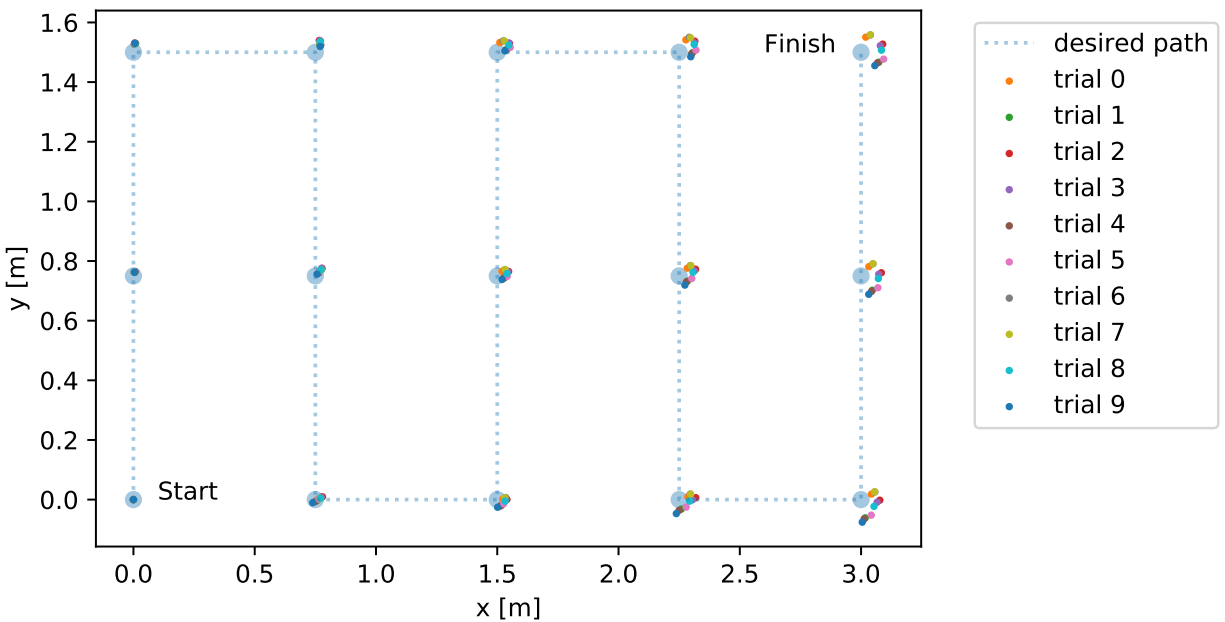
Figure 4.4: Position of the robot at each test point over the path moving in the positive x direction.
