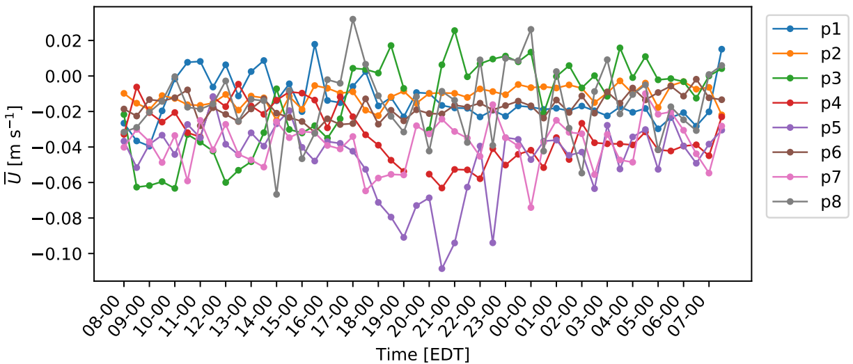
Figure 5.2: Average U component of the wind velocity vector over a diurnal cycle.
